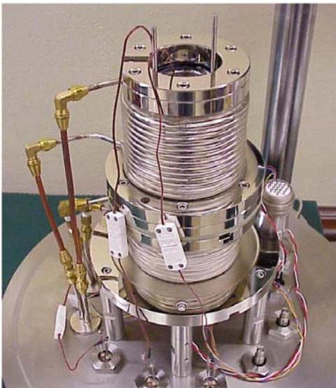
Figure 7. Attitude control wheel simulator test rig.
