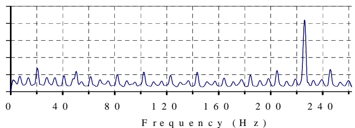
Figure 13. Accelerometer demodulation spectrum.
